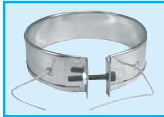
F Style Exiting on both sides of the gap
