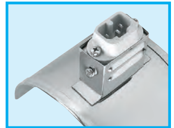
K3P Style 3 Prong with ground
