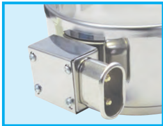
K90 Style Tangential with box
